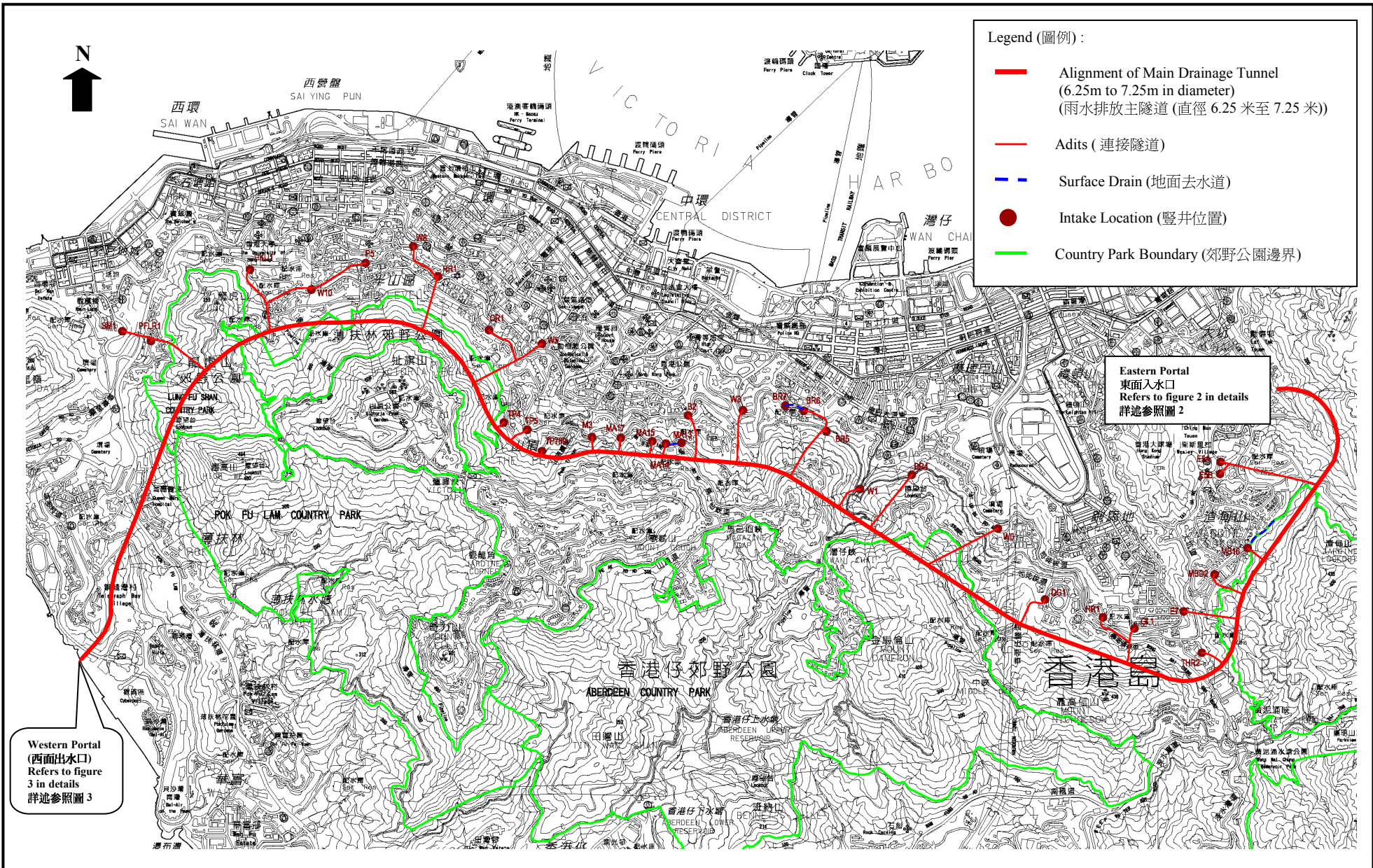
Figure 1: Locations of the main drainage tunnel, adits and intakes 圖 1 : 雨水排放主隧道, 連接隧道及豎井位置
